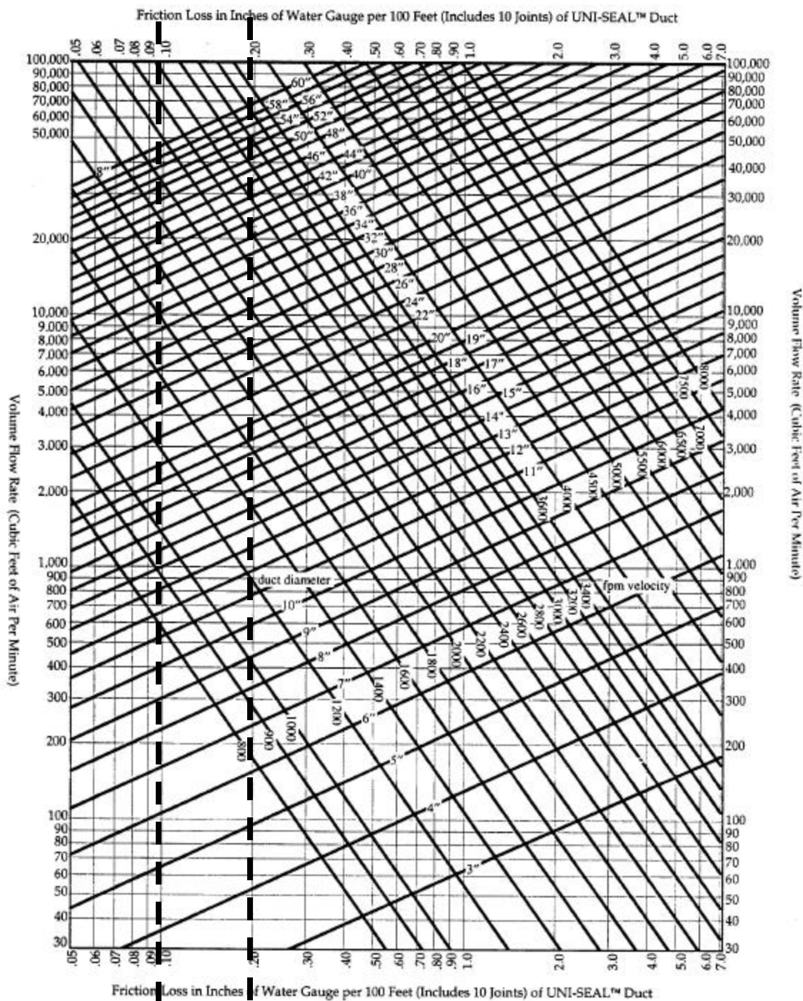
Figure 2.2 Friction Loss of Duct
